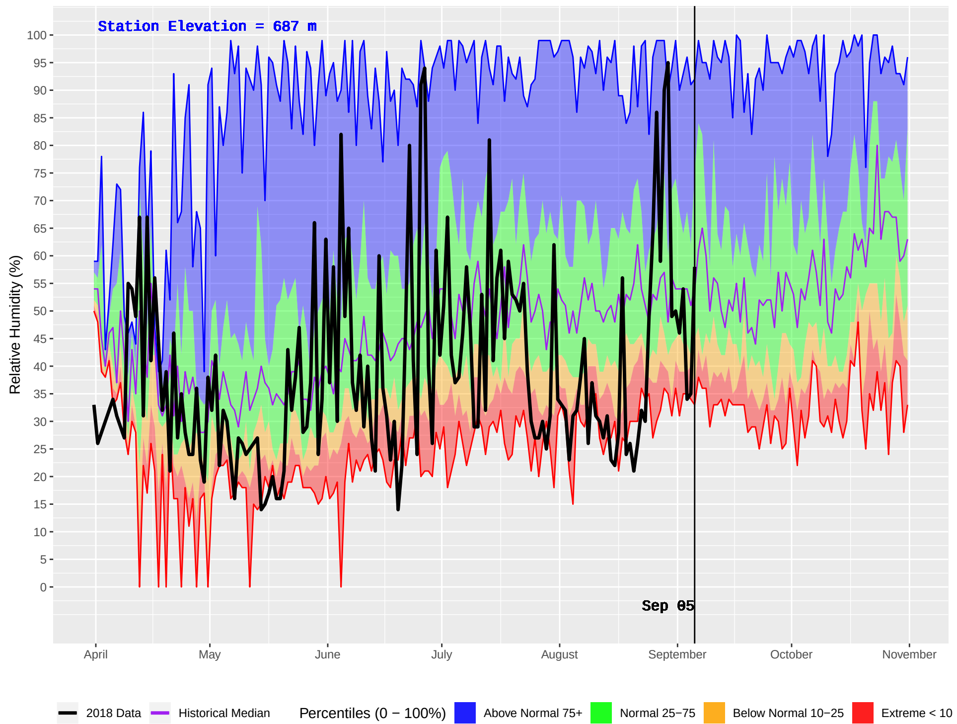
KETCHIKA (444) : Historical (1986–2016) and Current (2018) Daily Relative Humidity
