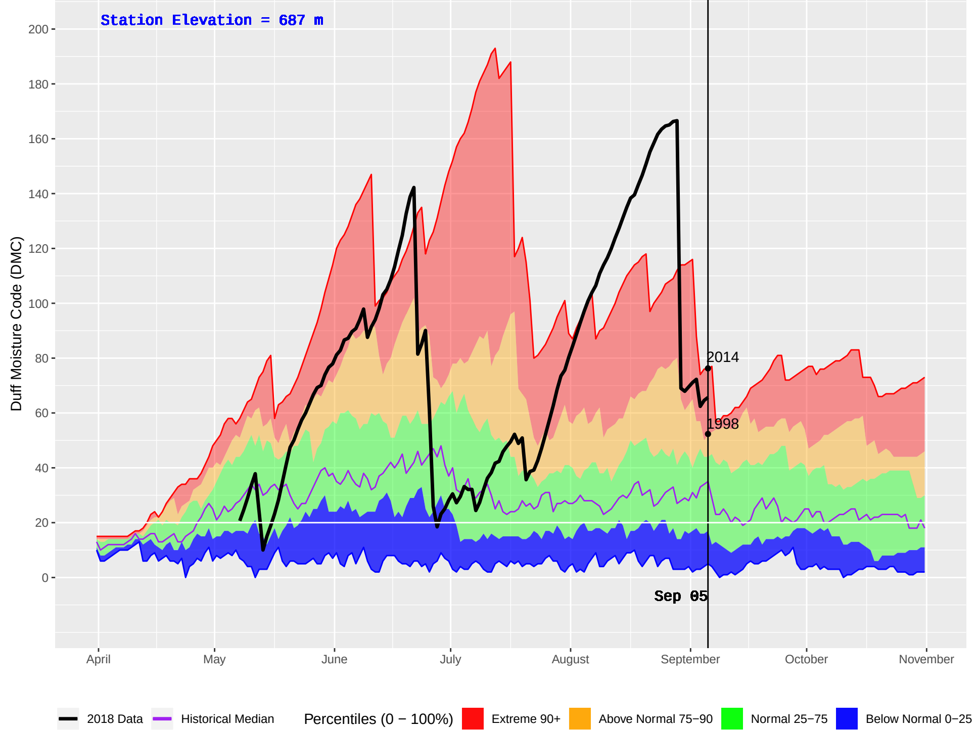
KETCHIKA (444) : Historical (1986–2016) and Current (2018) Daily Duff Moisture Code (DMC)
