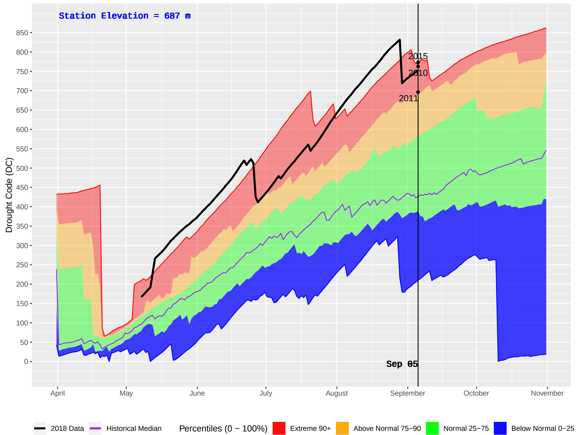
KETCHIKA (444) : Historical (1986–2016) and Current (2018) Daily Drought Code (DC)
