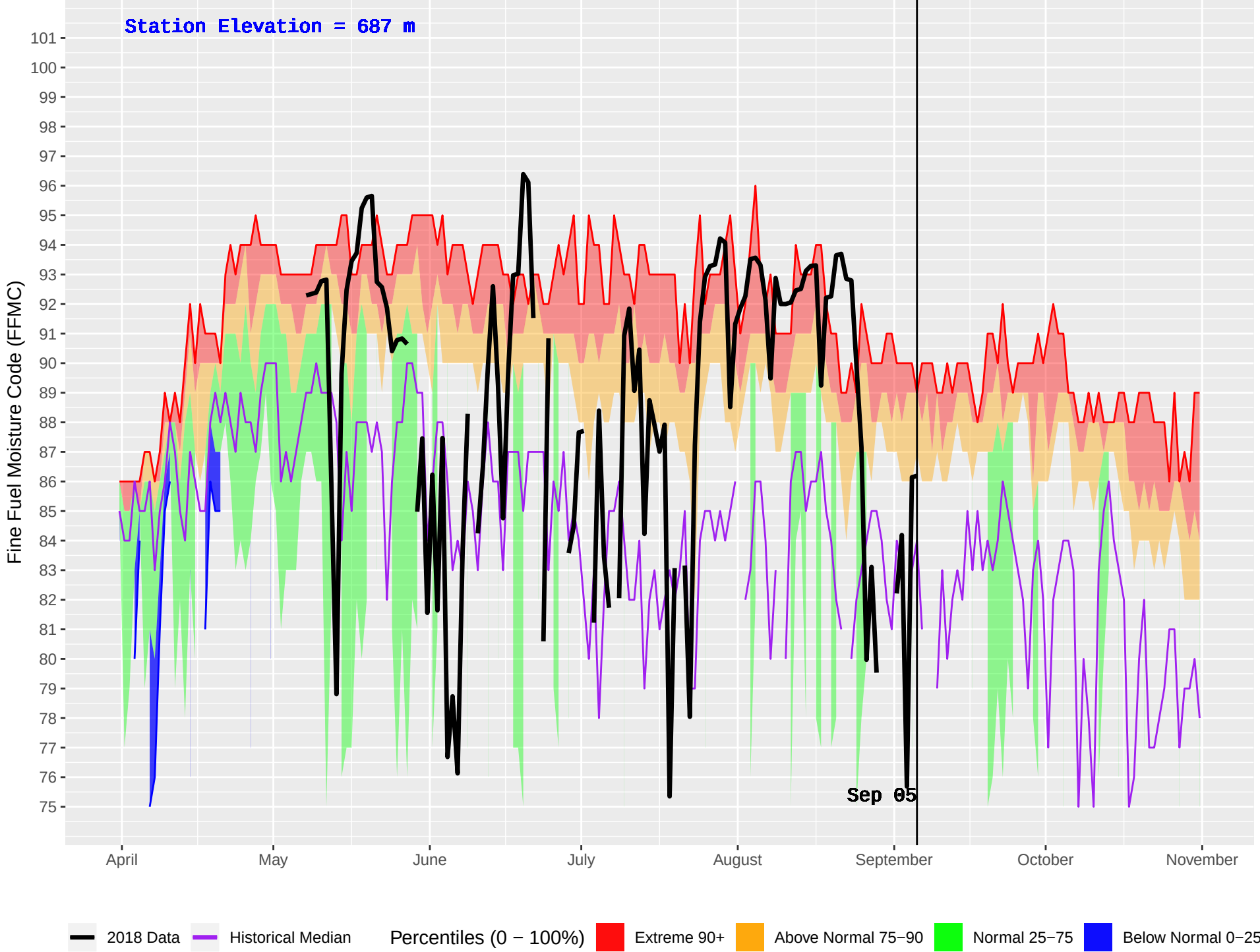
KETCHIKA (444) : Historical (1986–2016) and Current (2018) Daily Fine Fuel Moisture Code (FFMC)
