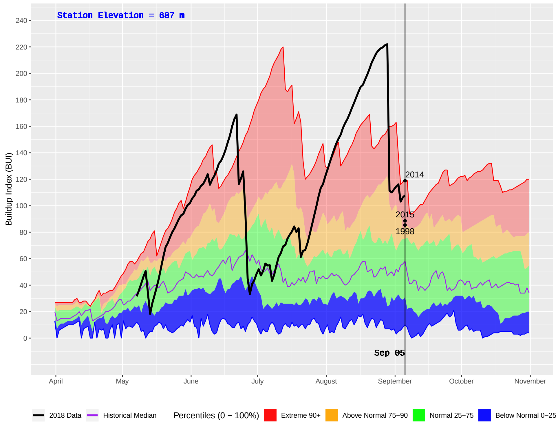
KETCHIKA (444) : Historical (1986–2016) and Current (2018) Daily Buildup Index (BUI)
