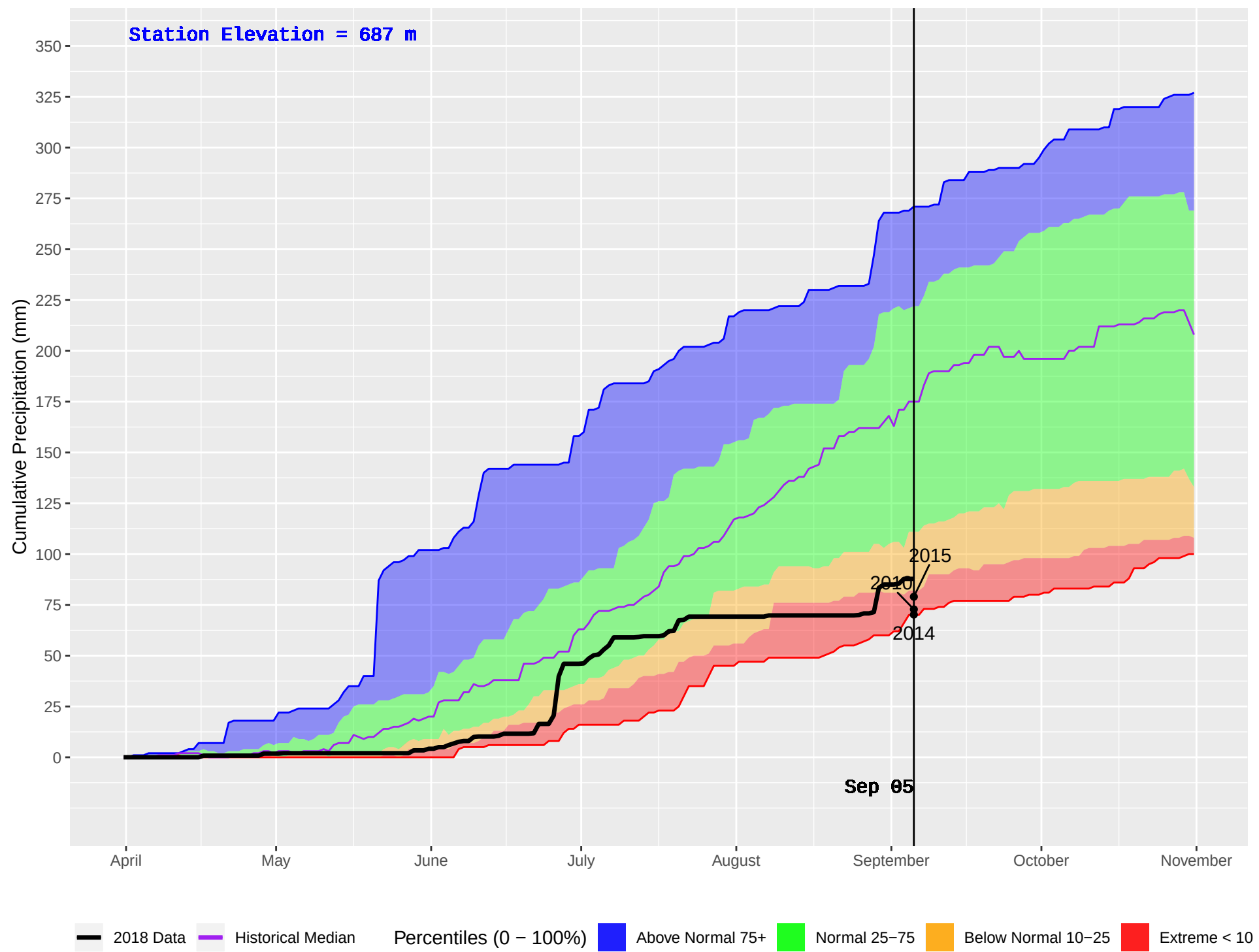
KETCHIKA (444) : Historical (1986–2016) and Current (2018) Daily Cumulative Precipitation
